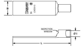
Figure 3. Blank Tongue
