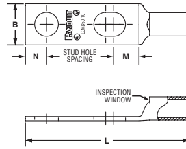
Figure 2. Two-Hole Slotted
