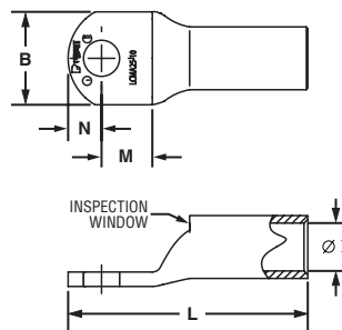
Figure 1. One-Hole
