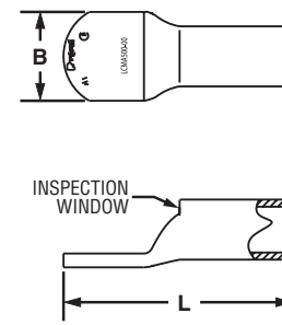
Figure 2. Blank Tongue
